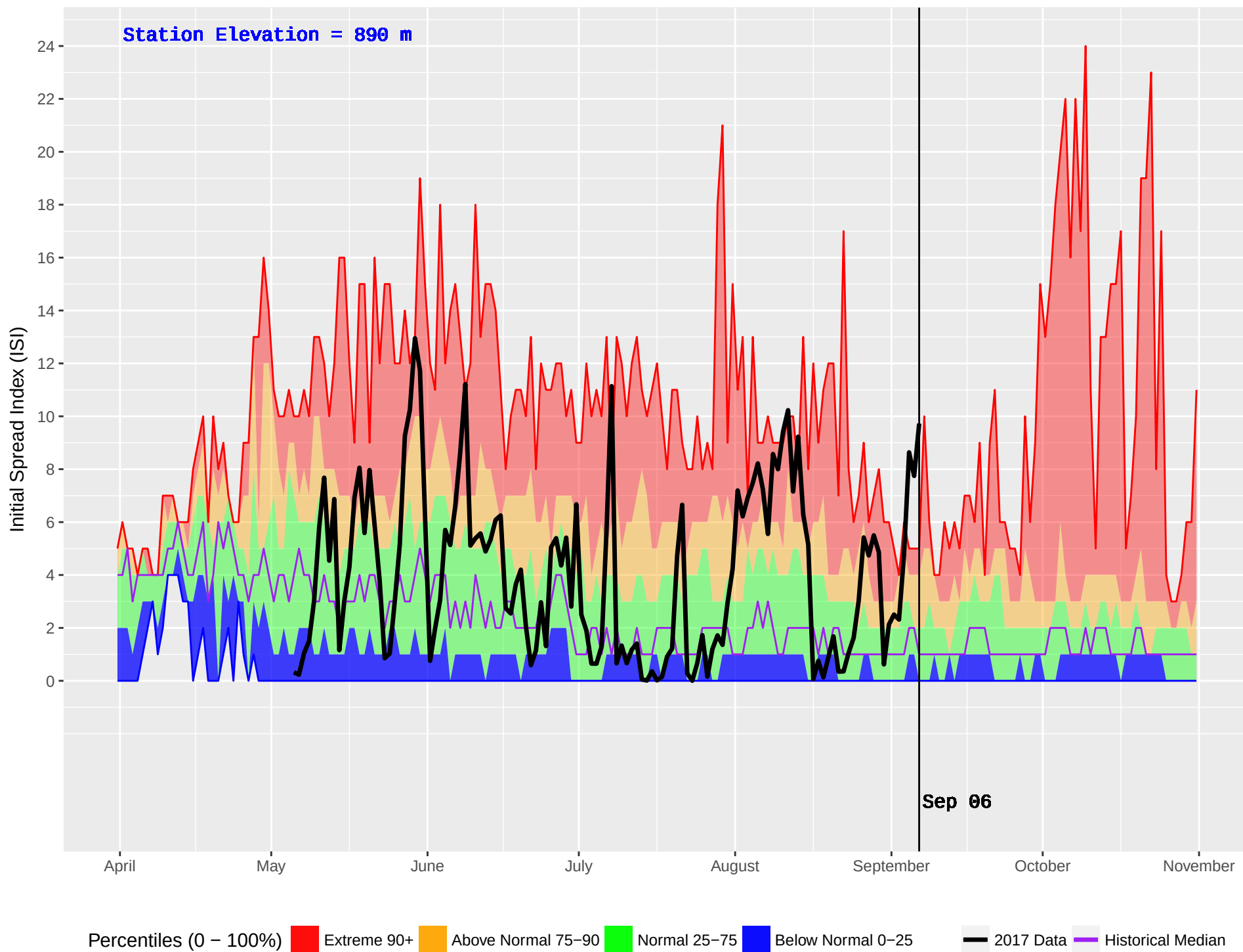
ISKUT (112) : Historical (1979–2016) and Current (2017) Noon Initial Spread Index (ISI)
