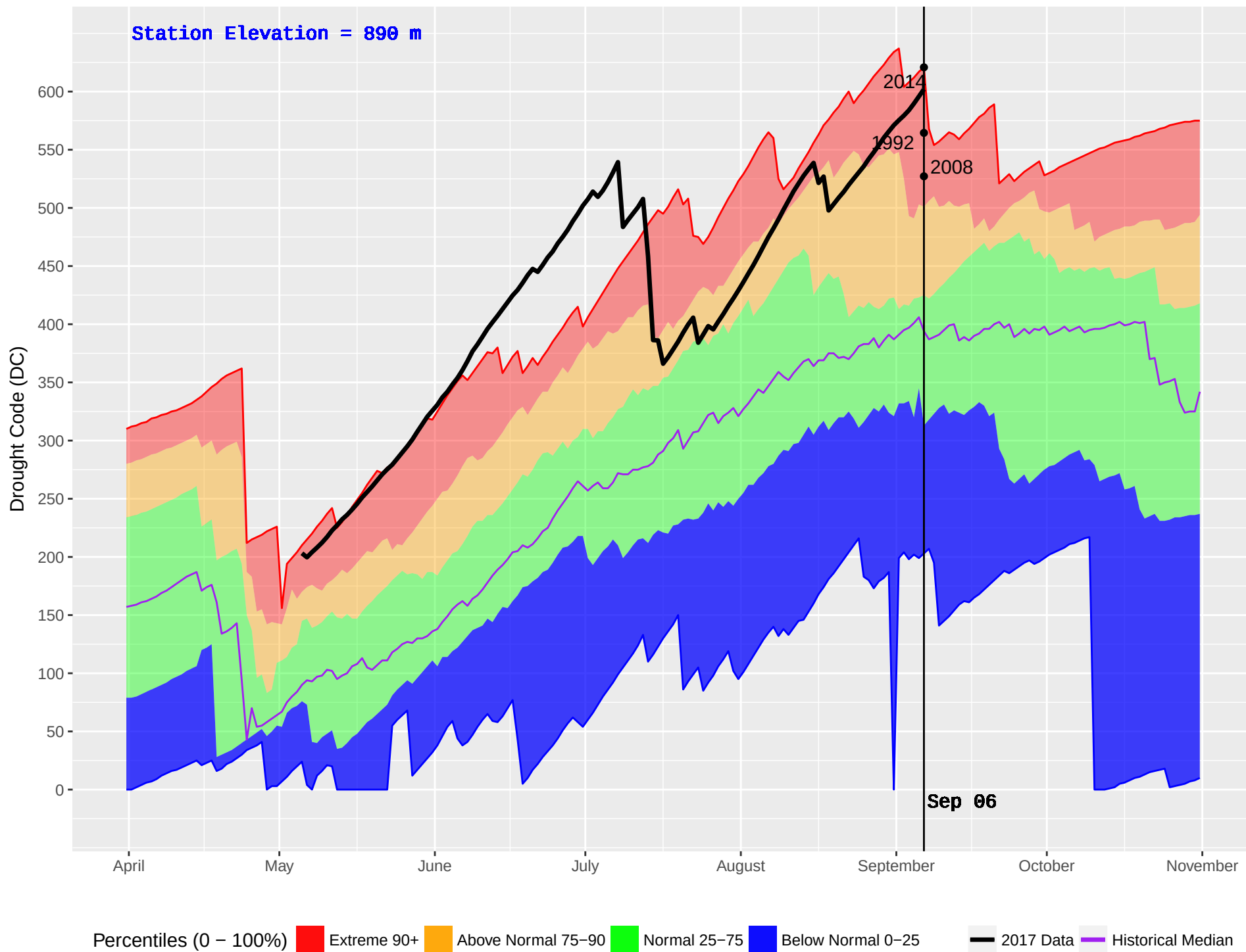
ISKUT (112) : Historical (1979–2016) and Current (2017) Noon Drought Code (DC)
