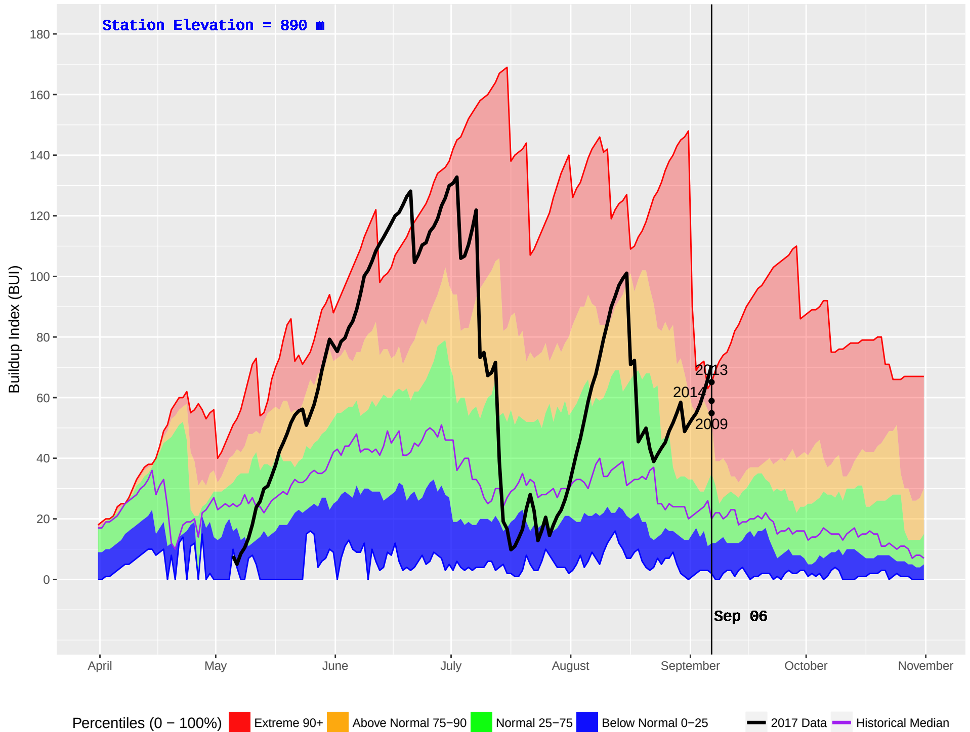
ISKUT (112) : Historical (1979–2016) and Current (2017) Noon Buildup Index (BUI)
